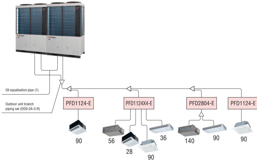
Outdoor unit's branch piping set
